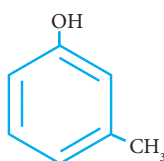
3-Methylphenol or meta methylphenol
