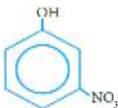
1,3 Nitro hydroxybenzene Meta-nitrophenol Meta-hydroxy nitrobenzene
