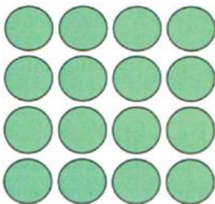
Diamagnetism
