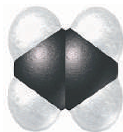
\text{H}_2\text{C}=\text{CH}_2 Ethylene Molecule
