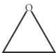
XIII Ethylene Epoxide
