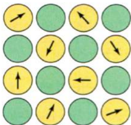
Paramagnetism
