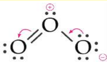
Composition I
