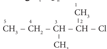
2-Chloro-3-methyl pentane
