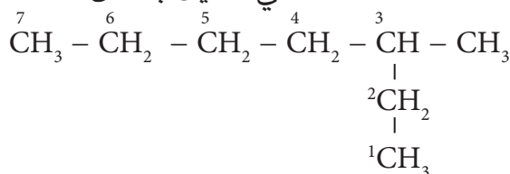
3-Methyl heptane
